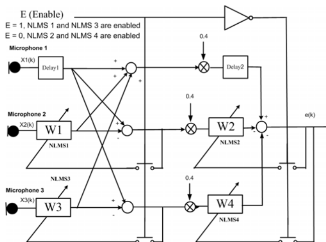
Fig. 3 Three-microphone noise canceller block diagram
