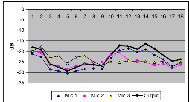
Fig. 12 Moving second voice (white noise) results
