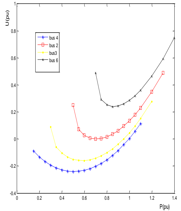
Fig. 5 QV Curves of 6-bus test system
