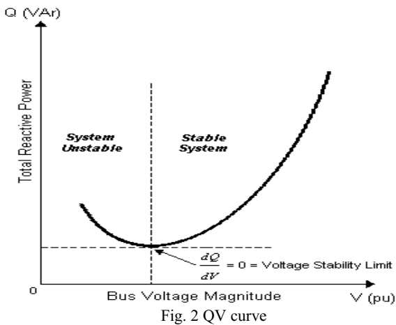
Fig. 2 QV curve
