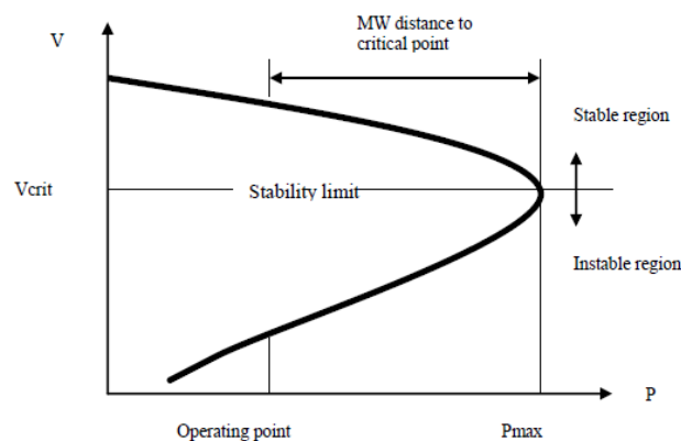
Fig. 1 PV curve
