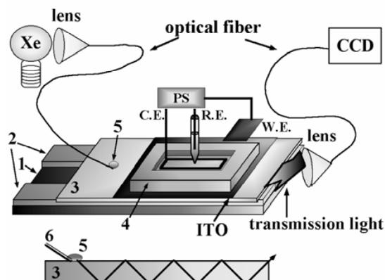
Fig. 1 Illustration of ITO-SOWG systems. 1: slide glass base, 2: silicon rubber strip acting SOWG supports, 3: SOWG (50 \times 20 \times 0.05 mm), 4: leak-proof silicone solution cell, 5: glycerol drop, and 6: optical fiber from the light source. PS: Potentiostat, W.E., C.E., and R.E.: working (ITO), counter (Pt wire), and reference (Ag/AgCl) electrode, and ITO: indium-tin-oxide electrode.
