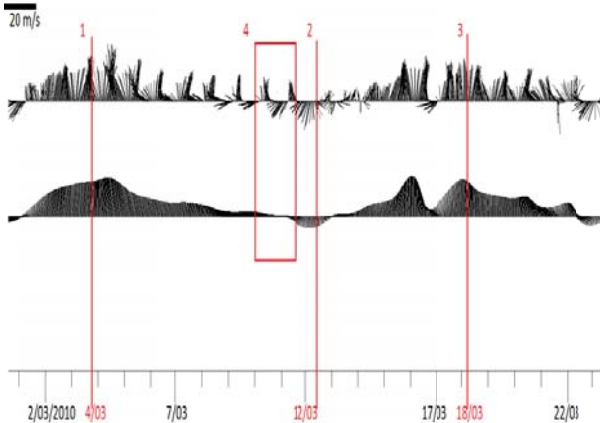
Fig. 4 Wind vector measured on Rottneet Island. Three wind incidents (04 March, 12 March and 18 March, 2010) are marked by a red solid line and numbered respectively
