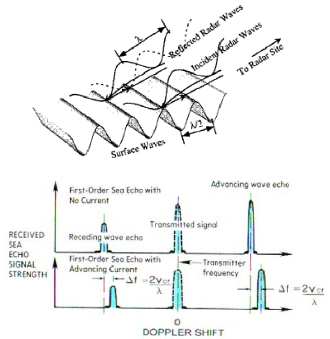
Fig. 2 Principle functionality of HF radars (Adapted from [9])
