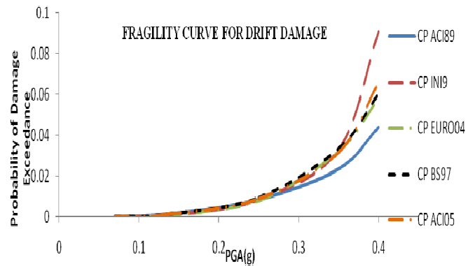
Fig. 3 Fragility curves for drift damage for 7 storey hospital building
