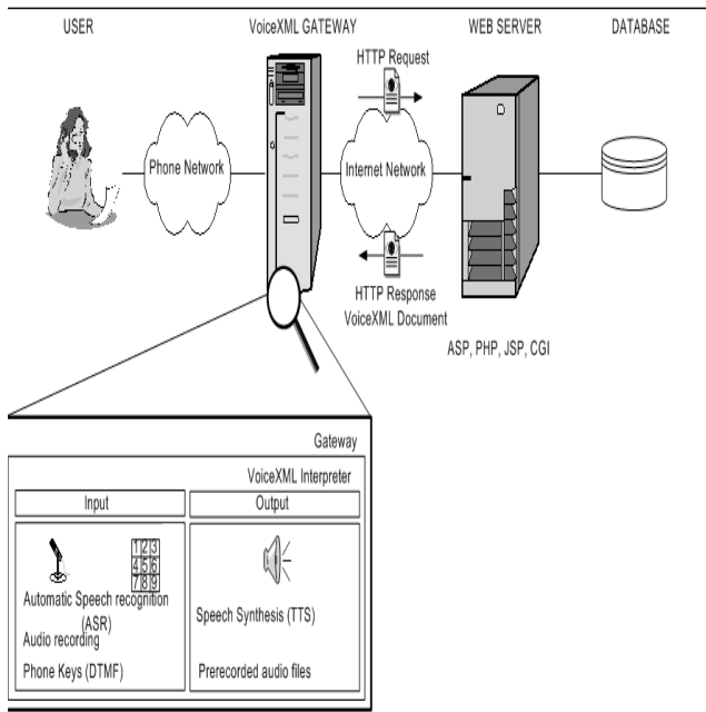
Fig. 1 VoiceXML Platform Architecture [20]
