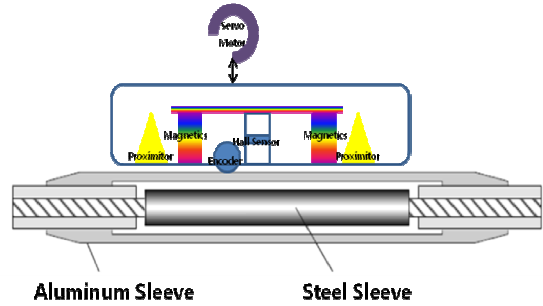
Fig. 8 Components diagram of inspection part
