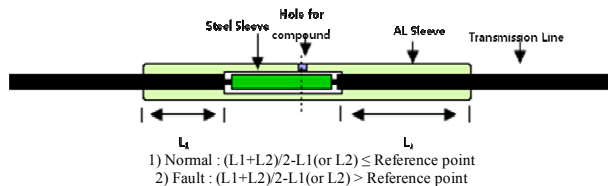
Fig. 15 Reference of normal & faulty line sleeve
