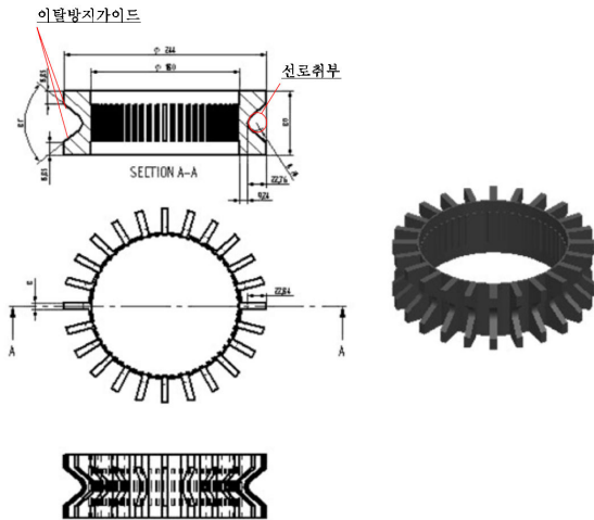
Fig. 5 Caterpillar adapted on moving part
