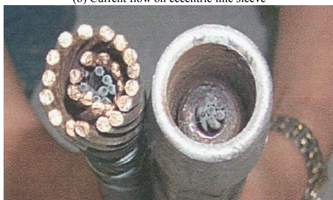
(c) Broken line sleeve cause of eccentricity Fig. 2 Line Sleeve current flow and broken sleeve
