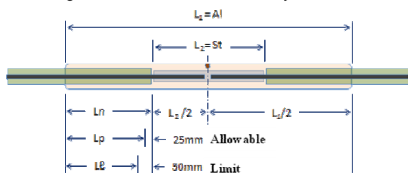
Fig. 15 Reference of normal & faulty line sleeve
