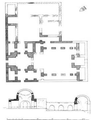
Fig.19 Plan and cross-section of “Roni” or “Rahni” building complex in Southeast of “Farashband”
