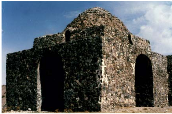
Fig.36 cross-vault "Baze-hur" after mending
