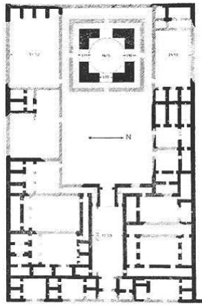
Fig.16 Plan of the fire-temple near KHosroparviz’s palace known as “Chahargapu” in Gasre Shirin
