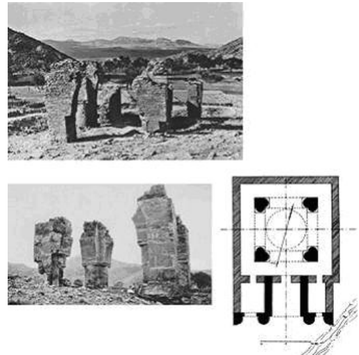
Fig.32 Exploration plan and some façades of the cross-vault "Atashkuh" (located on "Delijan-mahallat" route)
