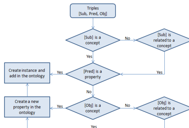
Fig. 3 Validation algorithm
