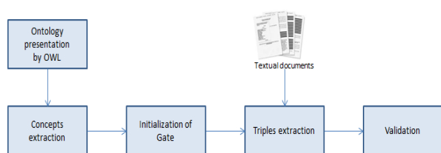
Fig. 2 Extraction algorithm from textual documents
