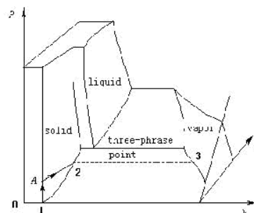
Fig. 1 p - v - T curves of matter
