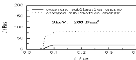
Fig. 4 The blow-off impulse induced by pulsed X-ray irradiating on aluminum, of which the energy spectrum is 3 keV blackbody spectrum, and the flux density is 200 J/cm 2
