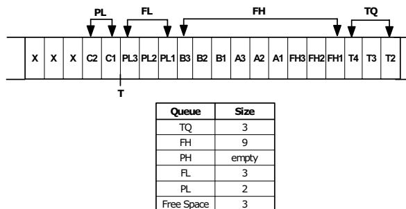
Fig. 8 The buffer state after dropping the packet
