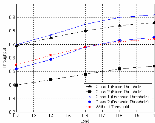
Fig. 12. Throughput versus load with buffer size =2000 cells.
