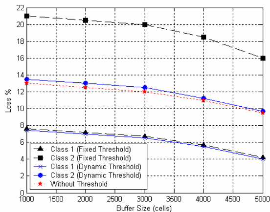
Fig. 11. Loss percentage versus buffer size at load =0.6.
