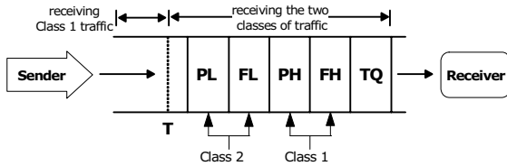
Fig. 1 Buffer Arrangement
