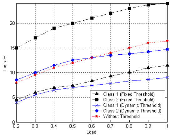
Fig. 10. Loss percentage versus load at buffer size =2000 cells.
