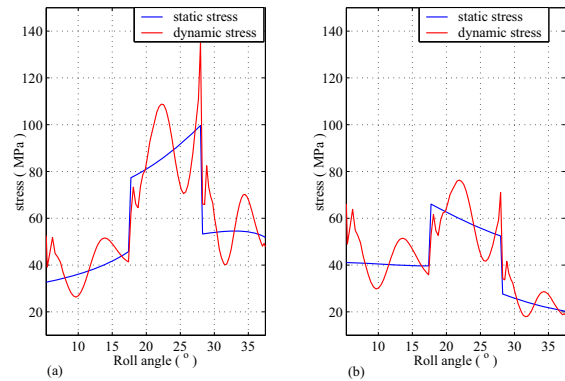
Fig. 7. Tooth bending stress as a function of the contact position for gears in stage I (gear train I), (a) pinion, (b) gear
