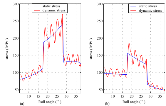
Fig. 8. Tooth bending stress as a function of the contact position for gears in stage II (gear train I), (a) pinion, (b) gear
