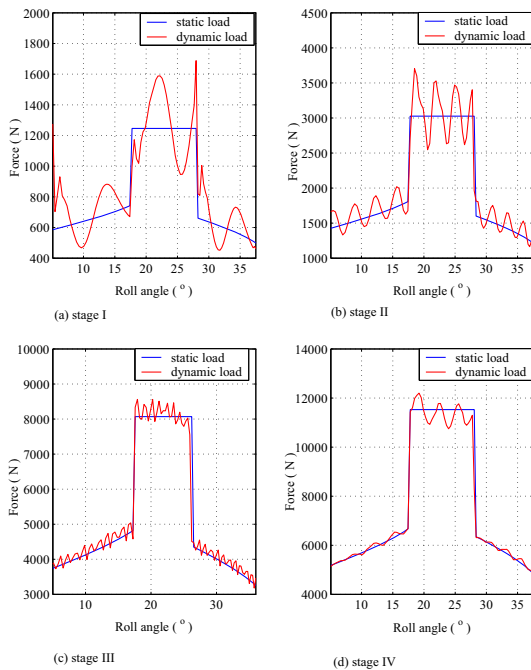
Fig. 6. Comparison of the dynamic and static load on a single tooth over the path of contact (gear train I)
