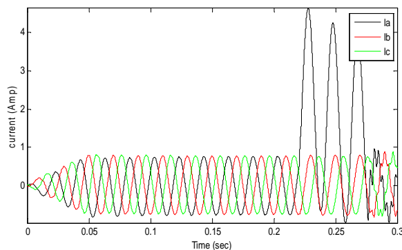
Fig. 3 Three phase currents for A-G fault
