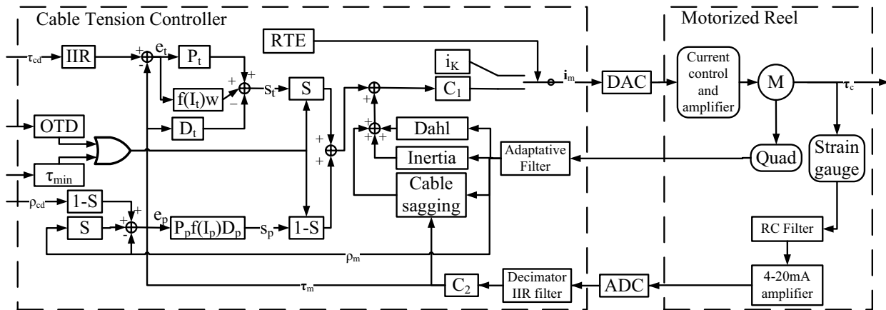
Fig. 7. Cable tension controller
