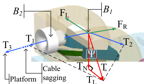
Fig. 4. Cable tensions and friction forces
