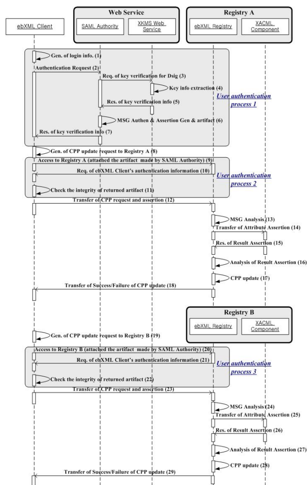
Fig. 4 Sequence Diagram – Scenario 1
