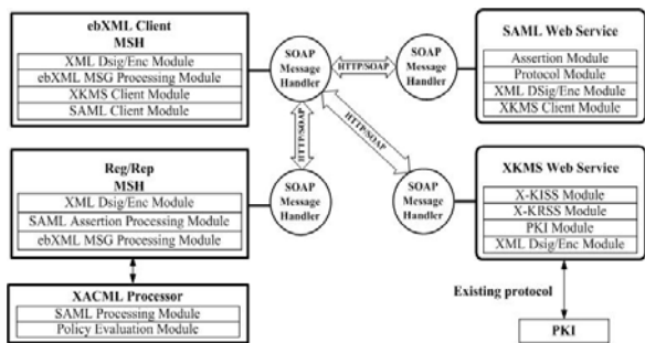
Fig. 7 Major Security Modules in the Test Software
