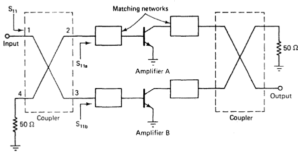
Fig.3, balanced amplifier configuration [2]
