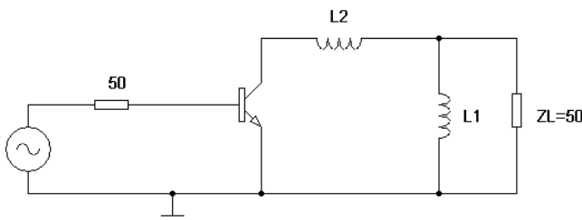
Fig.7, schematics diagram of a broadband amplifier
