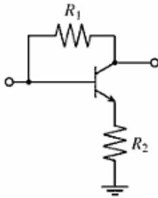
Fig.2, Negative resistive feedback circuits [1]
