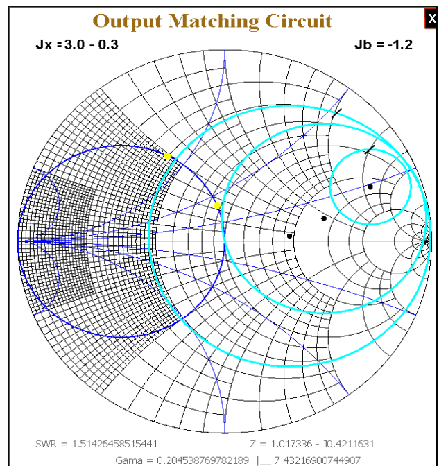
Fig.11, Output matching circuit with lumped elements
