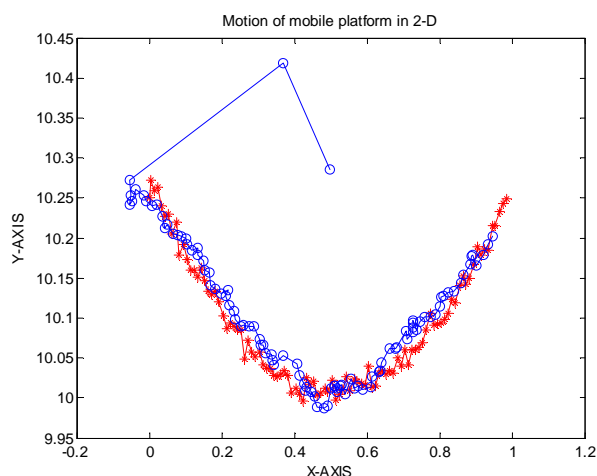
Fig. 6 Tracking Using Triangular Weighting Function
