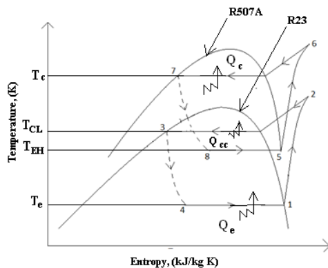
Fig.2 T-S diagram of cascade system
