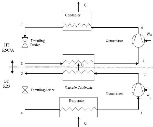
Fig.1 Schematic diagram of cascade system
