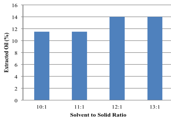
Fig. 3 Effect of solvent to solid ratio on amount of extracted oil at temperature 65°C and 9 hours extraction time
