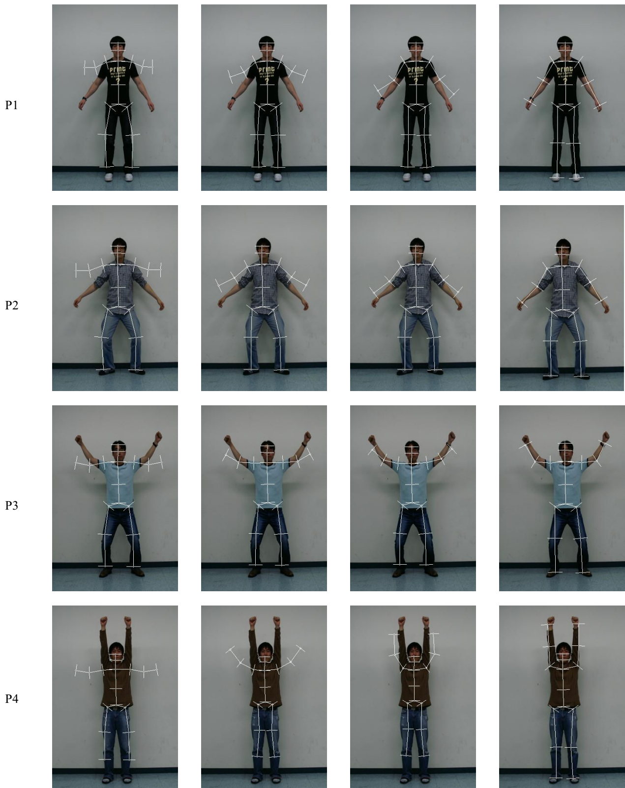
Fig. 5 Experimental results.
