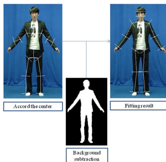
Fig. 4 Fitting process.
