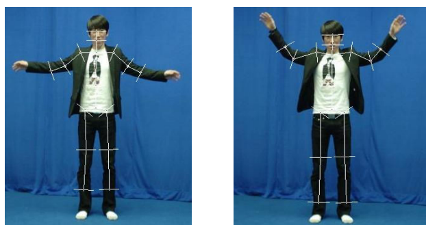
Fig. 3 Inaccurate results.
