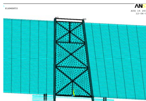
Fig. 4 The finite element model of Frame in ANSYS
