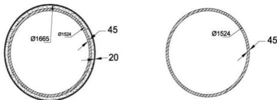
Fig. 2 Details of Leg and Pile Section (Unit: millimeter)
