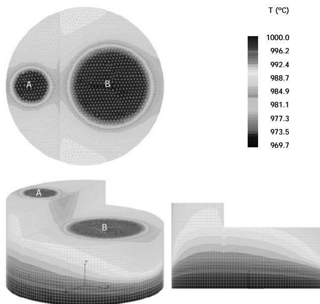
Fig. 8 Sample surface temperature distribution
