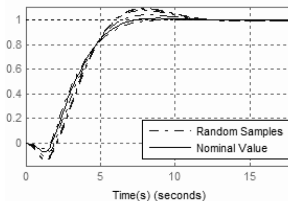
Fig. 10 Robustness of the H_{\infty} controller
