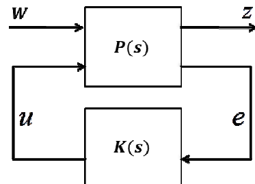
Fig. 5 Generalized plant
