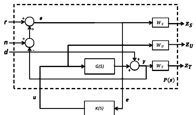
Fig. 4 General configurations for H_\infty control problems
