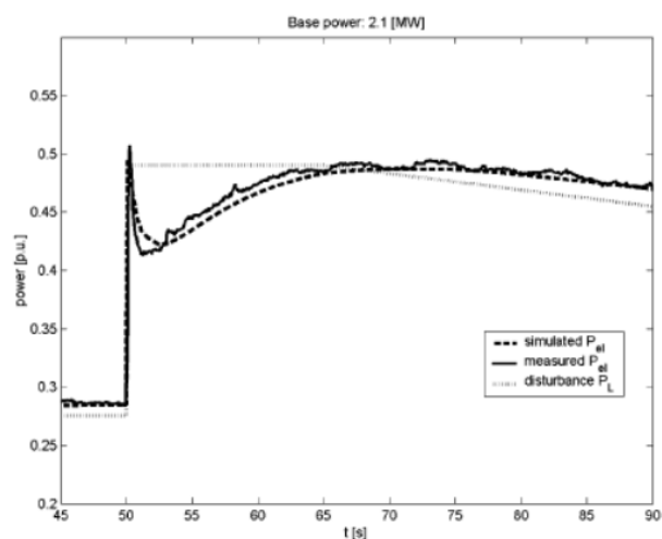
Fig. 7 Active Power with PID controller
