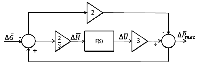
Fig. 3. Block diagram of the linear of turbine
