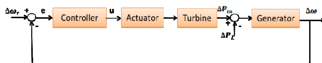
Fig. 1 Block diagram of speed control system
