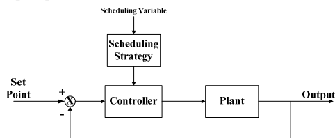
Fig. 1 Basic principle of gain scheduling control
