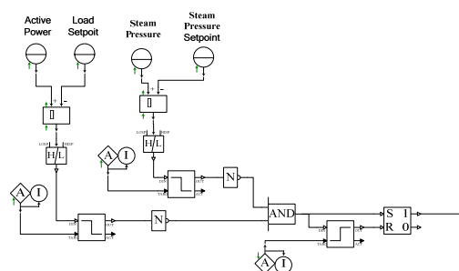
Fig. 2 Judgment of steady state operation
