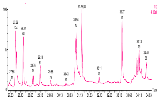
Fig.4. GC-MS chromatogram of the partially purified active fraction of A. marina leaf extract
