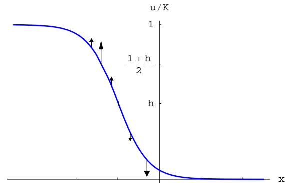
Fig. 6. A cartoon explaining the sharpness of the density profile in relation to hostility. The arrows indicate the direction and size of population growth at that location, due to the Allee effect.
