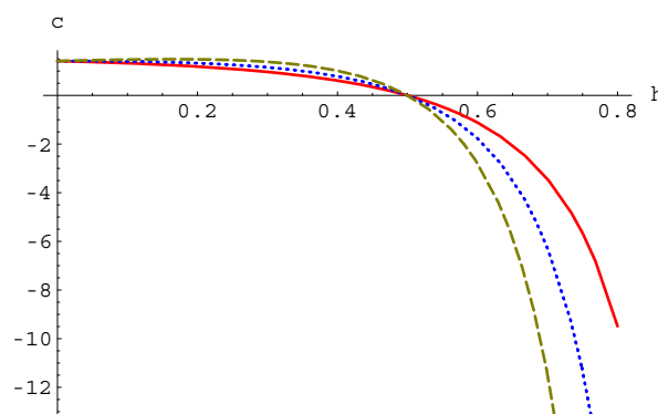
Fig. 8. Spreading speed in the presence of a hostility-influenced dispersal rate, as given in (12). The values r = 1 and \Phi = 1 are used, and the curves are drawn for n = 1 (solid), n = 2 (dotted), and n = 3 (dashed).
