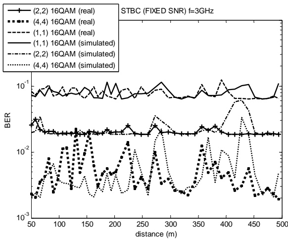
Fig. 8 Same as in Fig. 7 but with the OSTBC scheme for MIMO (2,2) and QSTBC for MIMO (4,4). Curves have been plotted using either measured or theoretical H matrices
