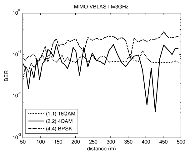
Fig. 7 Bit error rate along the tunnel with SISO, MIMO (2,2) and MIMO (4,4) and using the VBLAST scheme. The SNR is of 10 dB
