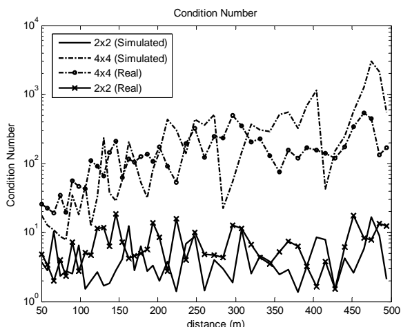
Fig. 6 Variation of the condition number of the H transfer matrix for a MIMO (2,2) or for a MIMO (4,4) configuration. The dotted lines and the continuous lines refer to values deduced from measurements or from the theoretical modelling, respectively
