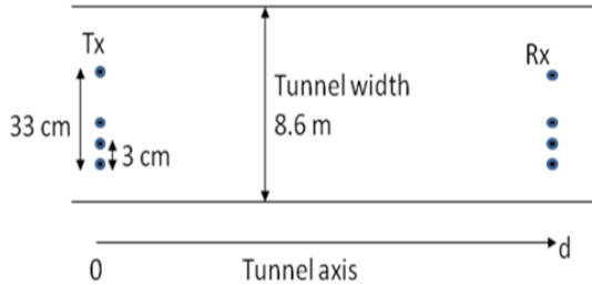
Fig. 1 Configuration of the virtual Tx/Rx arrays inside the tunnel
