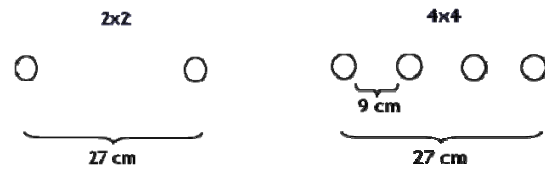
Fig. 4 Configuration of the antenna array for MIMO (2,2) and MIMO (4,4)
