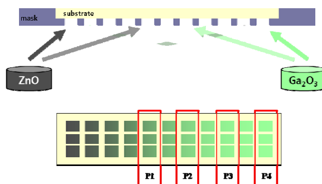
Fig. 1 A schematic diagram of combinatorial sputtering system
