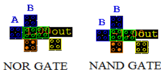
Fig. 9 NOR Gate and NAND Gate Layout
