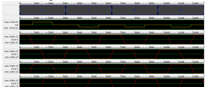
Fig. 17 Simulation result of NOR Gate
