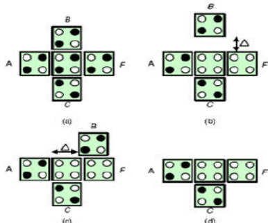
Fig. 6 (a) Defect-free majority gate, (b) displacement defect, (c) misalignment defect, and (d) omission defect.
