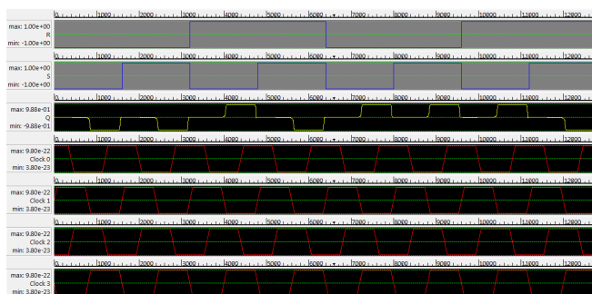
Fig. 21 Simulation result of SR Latch
