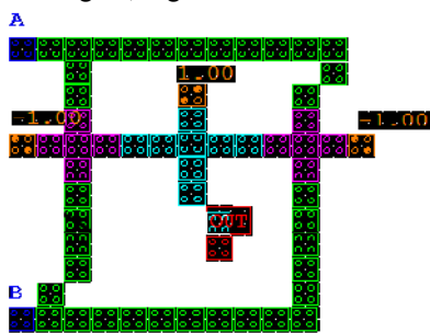
Fig. 10 XNOR Gate Layout
