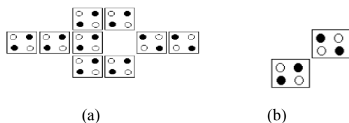
Fig. 4 (a) QCA Inverter (b) 2-cell QCA Inverter
