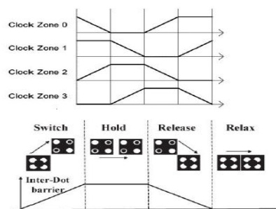
Fig. 7 The four phases of QCA Clock
