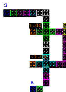
Fig. 13 SR Latch
