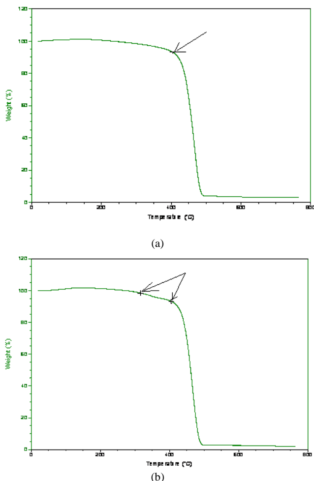
Fig. 4 TGA graphics, a- nanofiber without CNW, b- composite nanofiber with CNW which is produced by single nozzle and polymer solution without water
