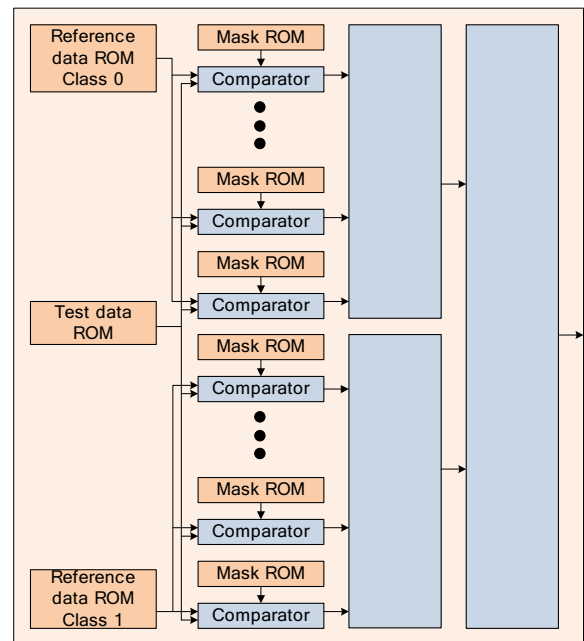
Fig. 3 DNAC processor architecture
