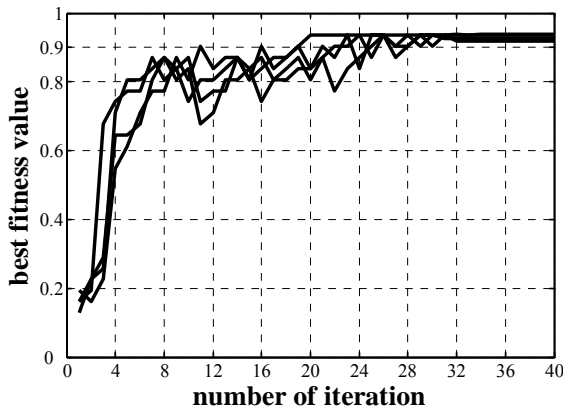
Fig. 3 Best fitness values of the proposed PSO-based estimator for three different try, over forty iterations, p = 100 , Y = 10 , and SNR = -5dB , p_c = 0.2 , and p_m = 0.1
