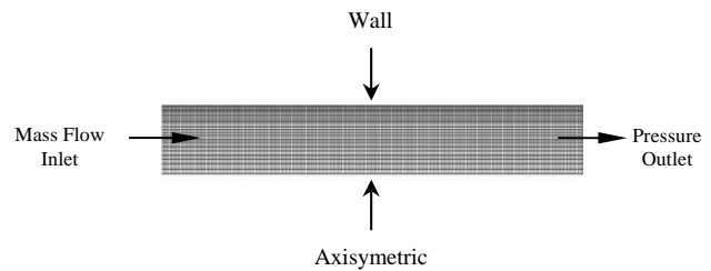
Fig. 2 Grid configuration with boundary conditions
