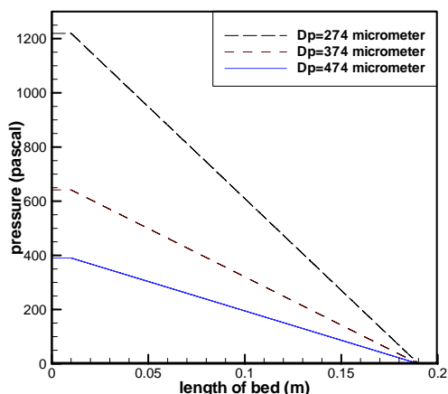
Fig. 3 Pressure drop through the simulated bed
