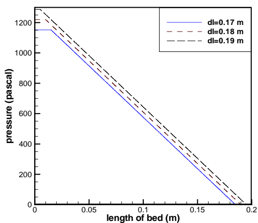
Fig. 4 Pressure drop through the simulated bed
