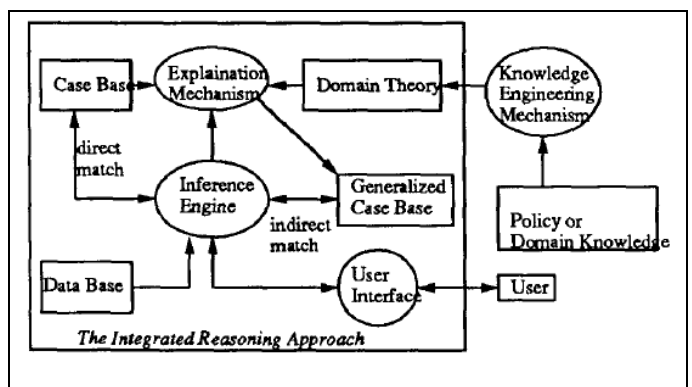
Fig. 1. A Model for Integrated Reasoning Approach [11]
