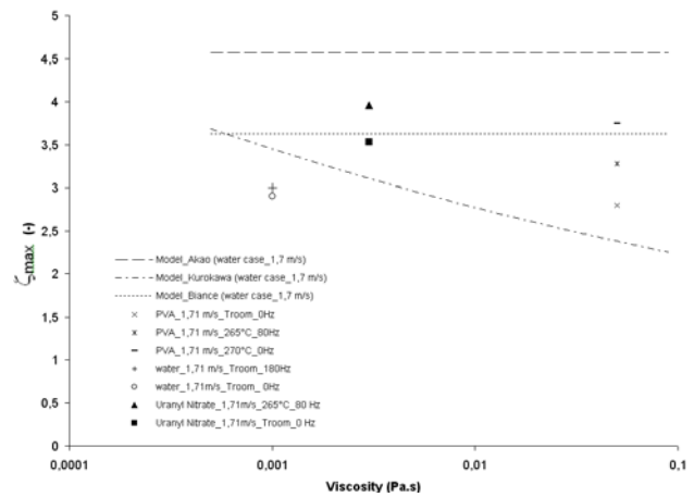
Fig. 12: Maximal values of \zeta_{max} as a function of the viscosity
