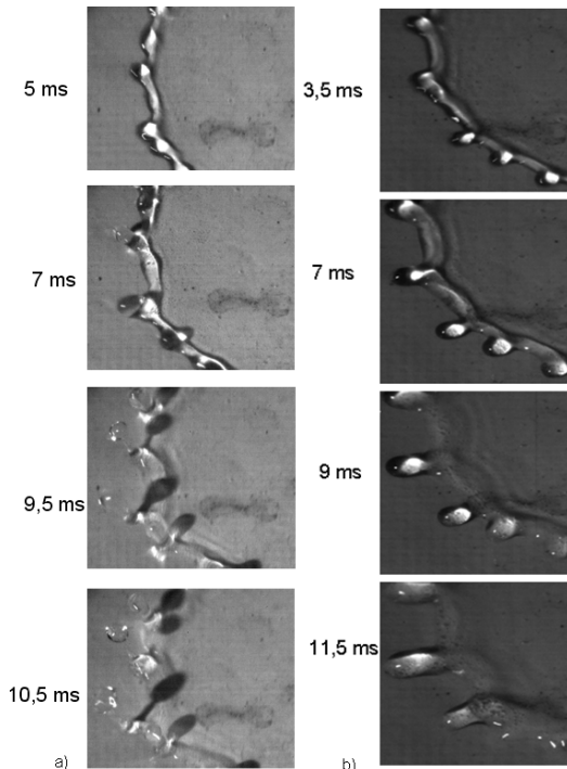
Fig. 15: Secondary fragmentation controlled by vibration of the surface impact after the spreading of a drop. ( f = 80 \text{ Hz} ; T=260^\circ\text{C} , Re = 7300 ) ; in Fig b), the spreading in the same conditions without vibration which does not break up the fingers
