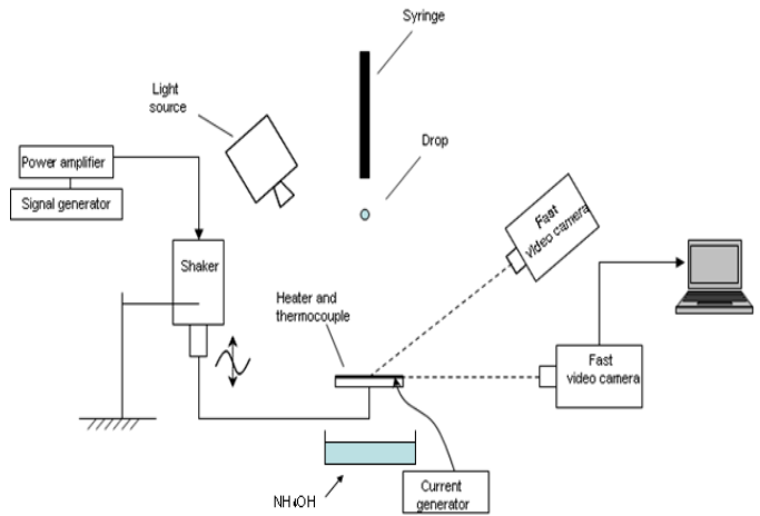
Fig. 9: Simplified diagram of the experimental set-up
