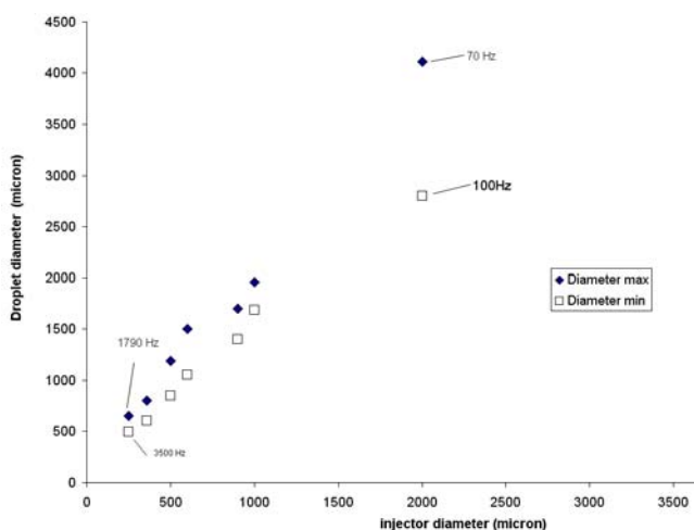
Fig. 2: Variation in the diameter of droplets obtained by passing through an aqueous PVA solution with a viscosity of 65 cP (18°C) via a vibrating injector with a variable-opening diameter. The diamonds show the maximum values obtained while the squares show the minimum values within a frequency range of 70 to 3.5 kHz.
