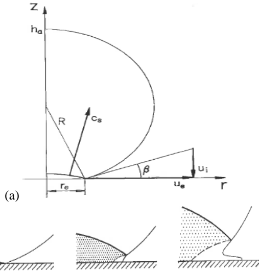
Fig. 4: Impact of a droplet on a solid surface: (a) initial stage, (b) propagation of a shock wave in the droplet after the initial step and its expansion until the onset of sideways jetting [11]
