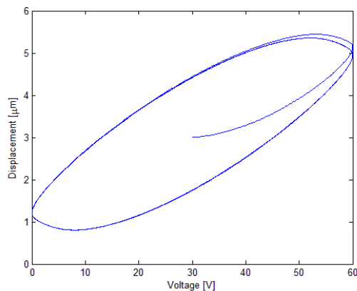
Fig. 1. Hysteresis loop with a sinusoidal voltage input
