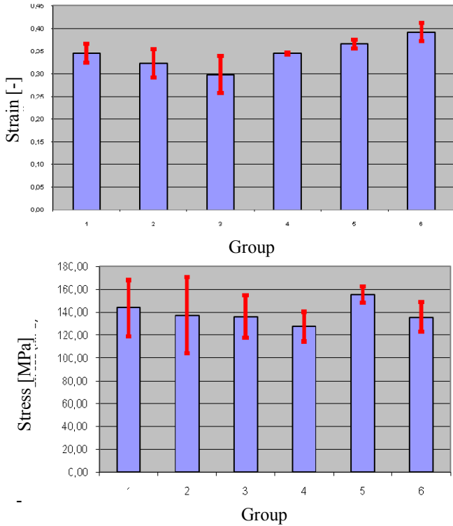
Fig. 4 Stress/Strain Results of Uniaxial Tests at Failure
