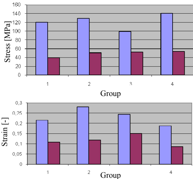
Fig. 5 Stress/Strain Data of Groups of Planar Biaxial Tensile Test
