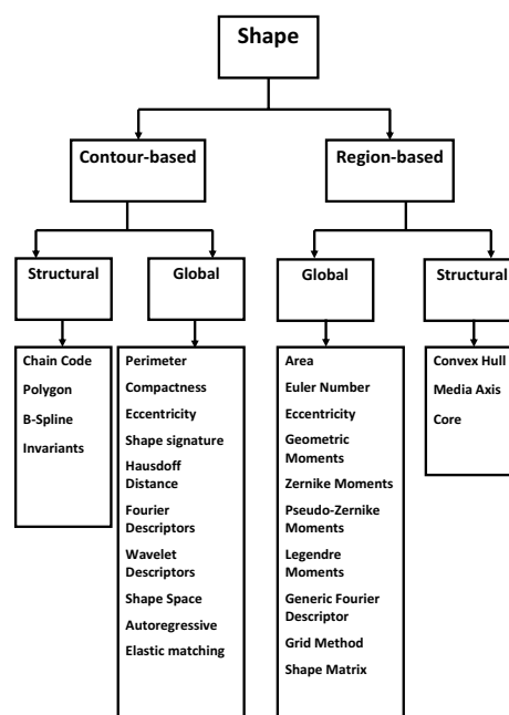
Fig. 1. Classification of shape representation and description techniques
