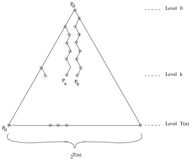
Fig. 1. Computation tree
