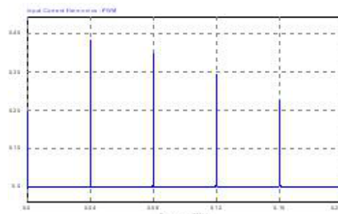
Fig. 8. Input Current Harmonic Spectrum - PWM Converter
