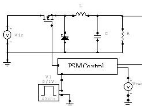
Fig. 1. Pulse Skipping Modulated Buck Converter
