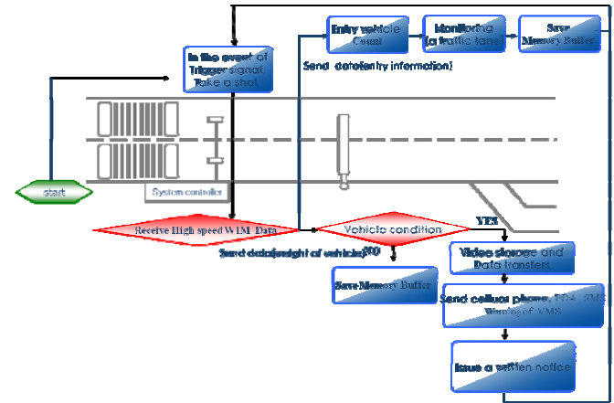
Fig. 4 System algorithm
