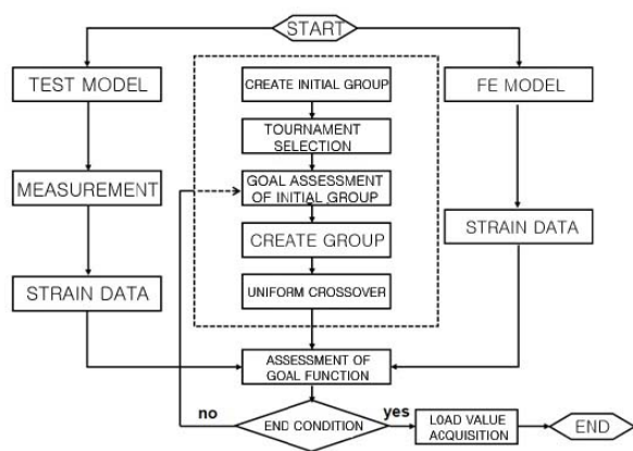
Fig. 4 The vehicle load analysis system
