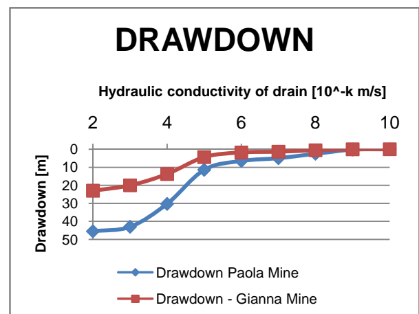
Fig. 5 Drawdown versus the hydraulic conductivity of the tunnel profile (a) Paola Mine, (b) Gianna Mine
