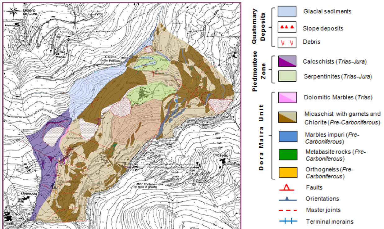
Fig. 2 Geological map of the study area
