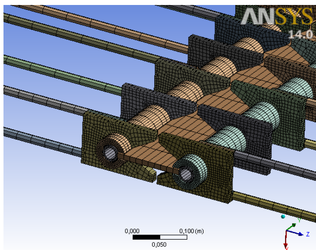
Fig. 1 Detail of computational model of static test
