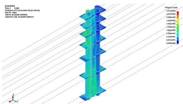
Fig. 11 Field of shear stress in the steel structure of steel joint
