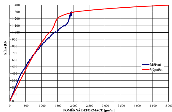
Fig. 3 Measured and calculated values of deformation
