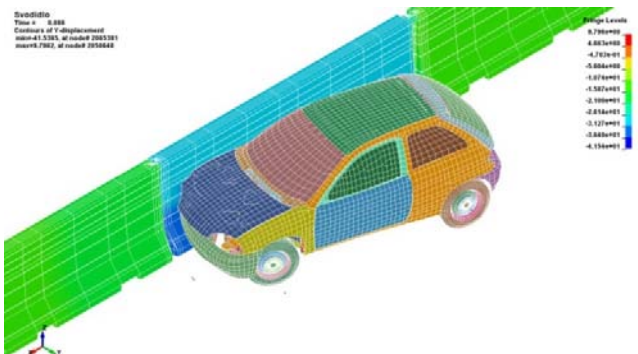
Fig. 10 The field of displacement of barrier
