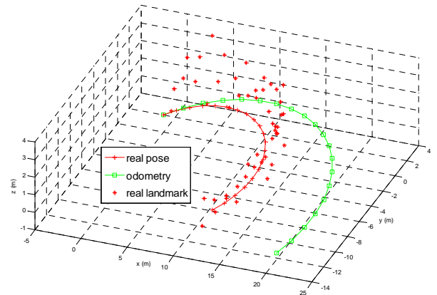
Fig.8. simulation environment
