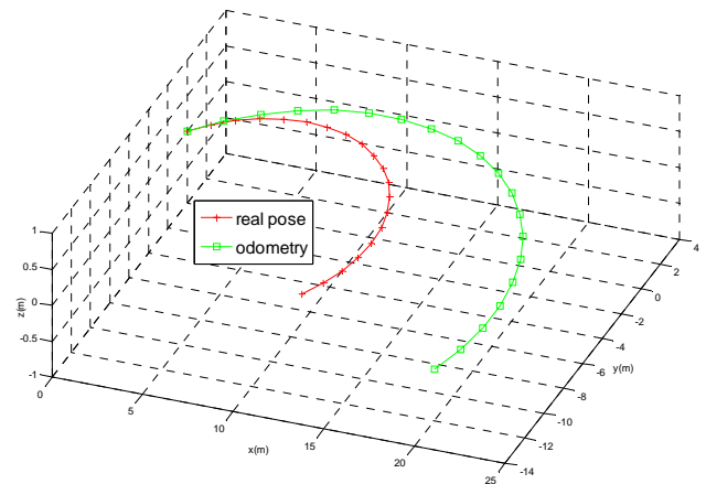
Fig. 2 Robot motion
