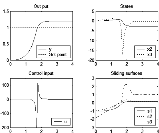
Fig3. Nested sliding mode control response for perturbed system with \varepsilon_1 = \varepsilon_2 = \varepsilon_3 = 10 .
