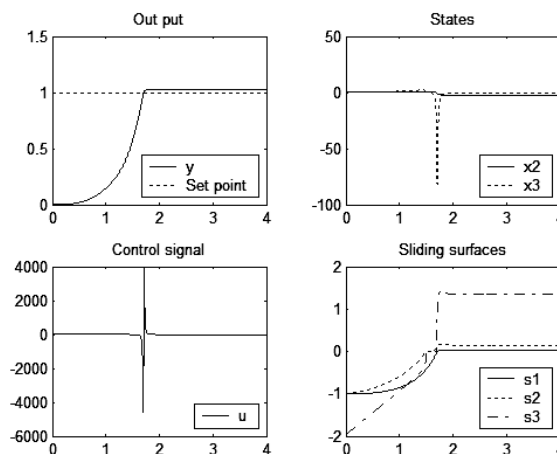
Fig4. Nested sliding mode control response for perturbed system with \varepsilon_1 = \varepsilon_2 = \varepsilon_3 = 50 .
