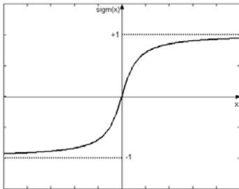
Fig1. sigm(x) as a continuous switch function
