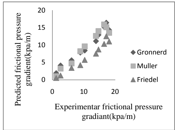
Fig. 15 Experimental frictional versus Predicted frictional pressure gradients for different methods, mass flow rate = 5.32 \cdot 10^{-5} kg/s . D_i = 0.6 mm and P_i = 3350 kpa
