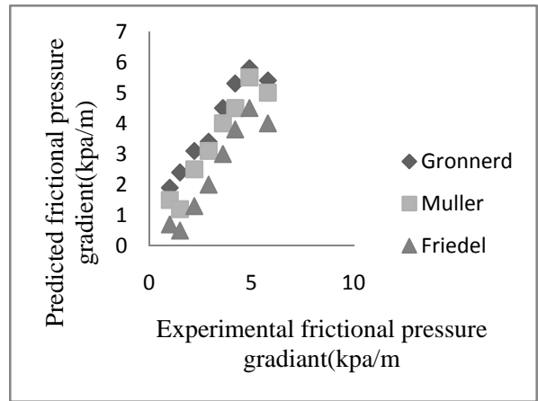
Fig. 14 Experimental frictional versus Predicted frictional pressure gradients for different methods, mass flow rate = 2.66 \cdot 10^{-5} kg/s . D_i = 1.6 mm and P_i = 3350 kpa
