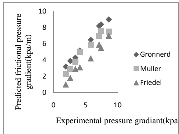
Fig. 16 Experimental frictional versus Predicted frictional pressure gradients for different methods, mass flow rate = 2.66 \cdot 10^{-5} kg/s . D_i = 1 mm and P_i = 3350 kpa
