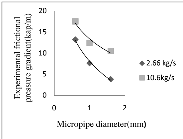
Fig. 3 Micro pipe (Di) Diameter versus frictional pressure gradient for different mass flow rates and P_i = 3350 kpa
