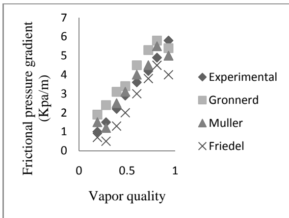
Fig. 12 Effect of vapor quality on the pressure gradient for D_i = 1.6 mm and mass flow rate = 2.66 \cdot 10^{-5} kg/s and P_i = 3350 kpa
