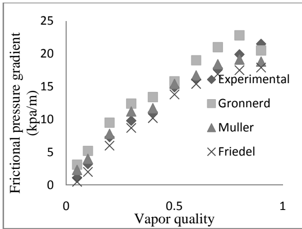
Fig. 11 Effect of vapor quality on the pressure gradient for D_i = 0.6 mm and mass flow rate = 8 \cdot 10^{-5} kg/s and P_i = 3350 kpa
