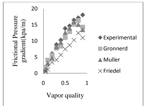
Fig. 9 Effect of vapor quality on the pressure gradient for Di = 1 mm and mass flow rate =5.32 \cdot 10^{-5} kg/s and Pi = 3350 kpa
