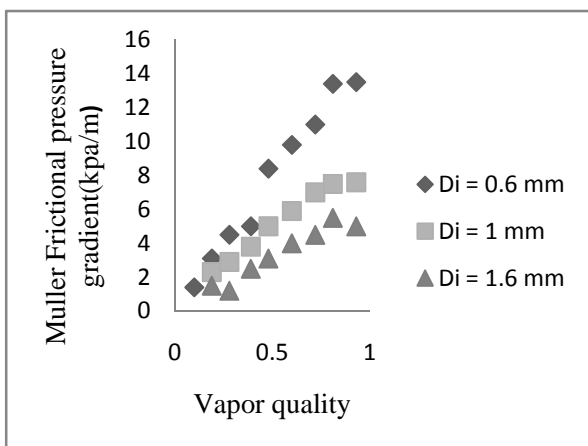
Fig. 7 Effect of vapor quality on the pressure gradient for Di = 0.6 mm and mass flow rate =2.66 \cdot 10^{-5} kg/s
