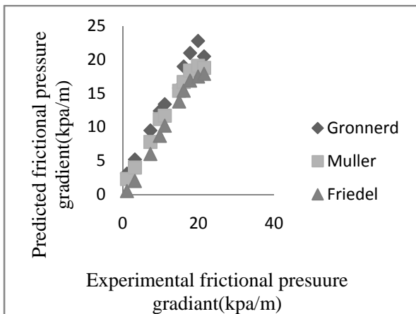
Fig. 13 Experimental frictional versus Predicted frictional pressure gradients for different methods, mass flow rate = 8 \cdot 10^{-5} kg/s . D_i = 0.6 mm and P_i = 3350 kpa
