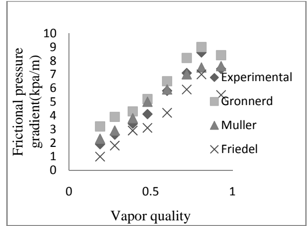
Fig. 8 Effect of vapor quality on the pressure gradient for Di = 1 mm and mass flow rate =2.66 \cdot 10^{-5} kg/s and Pi = 3350 kpa
