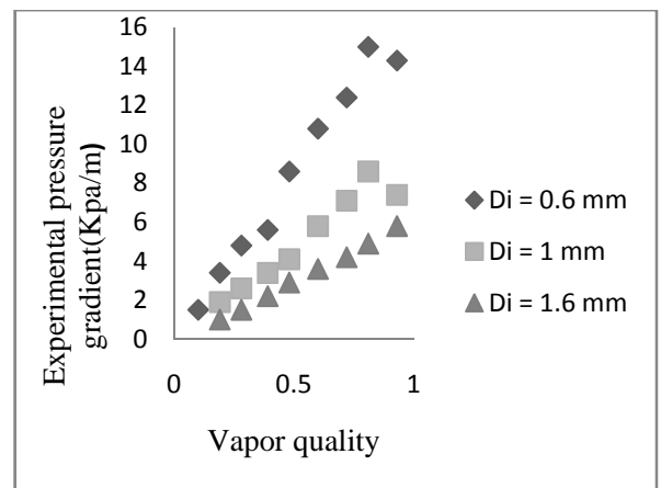
Fig. 10 Effect of vapor quality on the pressure gradient different Di, mass flow rate =2.66 \cdot 10^{-5} kg/s and Pi = 3350 kpa
