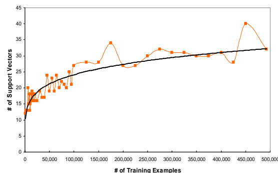
Fig. 5 SVM-Perf Number of Support Vectors vs. Training Data Size
