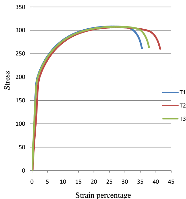
Fig. 7 Stress – Strain Curve
