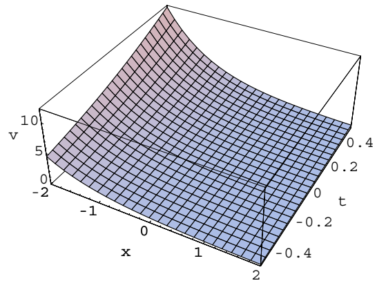
Fig. 7: (Ex.3, Exact solution v = e^{t-x} )
