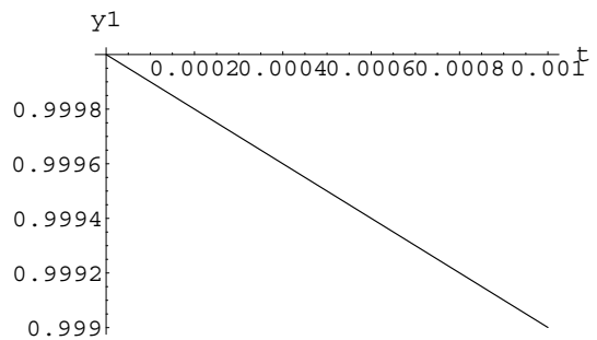
Fig. 8: (Ex.4, 3-term solution y_1 )
