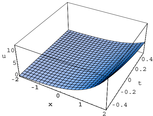
Fig. 5: (Ex.3, Exact solution u = e^{x-t} )
