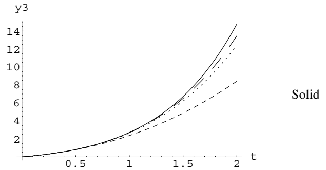
Fig. 3: (Ex.2, y_3 ) line = exact solution, dashed line = standard NIM, long dashed line = revised ADM, dotted line = revised NIM
