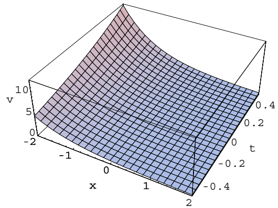
Fig. 6: (Ex.3, 3-term solution v )
