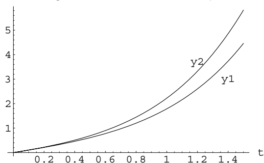
Fig. 11: (Ex.5, 4-term solutions)
