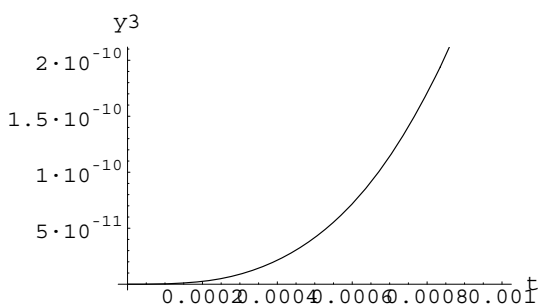
Fig. 10: (Ex.4, 3-term solution y_3 )
