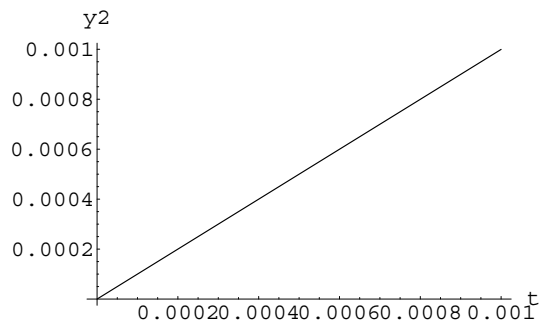
Fig. 9: (Ex.4, 3-term solution y_2 )
