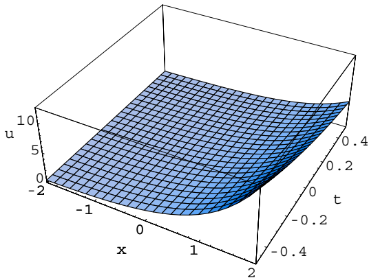
Fig. 4: (Ex.3, 3-term solution u )
