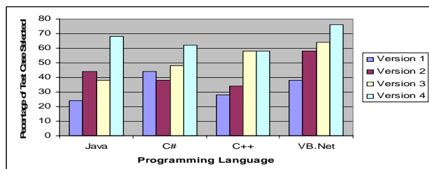
Fig. 7 Percentage of test cases selected for Sorting Software
